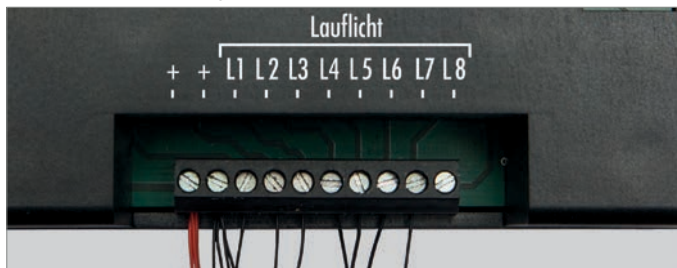
Fig. 22: Connecting warning lights/construction site barrier
