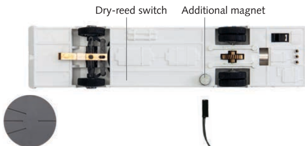
Fig. 26: H0 Underbody
