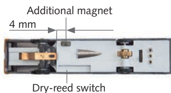
Fig. 27: N Underbody
